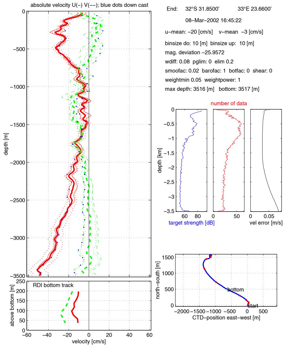
Figure L12: DWH velocity, data quality and ship drift processed using Visbeck method without bottom-tracked velocity constraint
