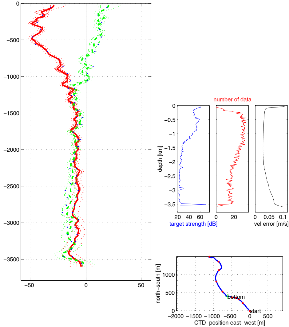
Figure L8: BB velocity profiles, data quality, and ship drift processed using Visbeck method
