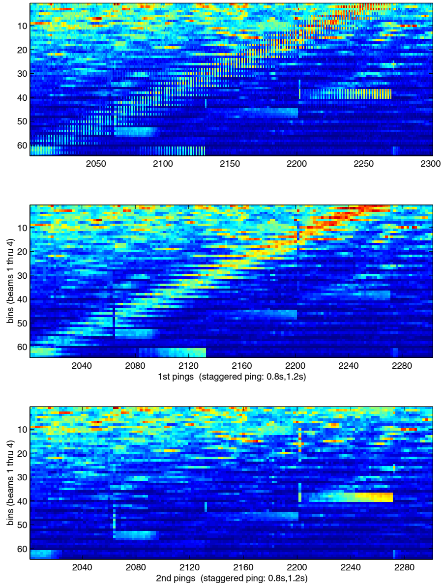
Figure L3: Solo BB deployment: Detail of Beam Amplitudes
