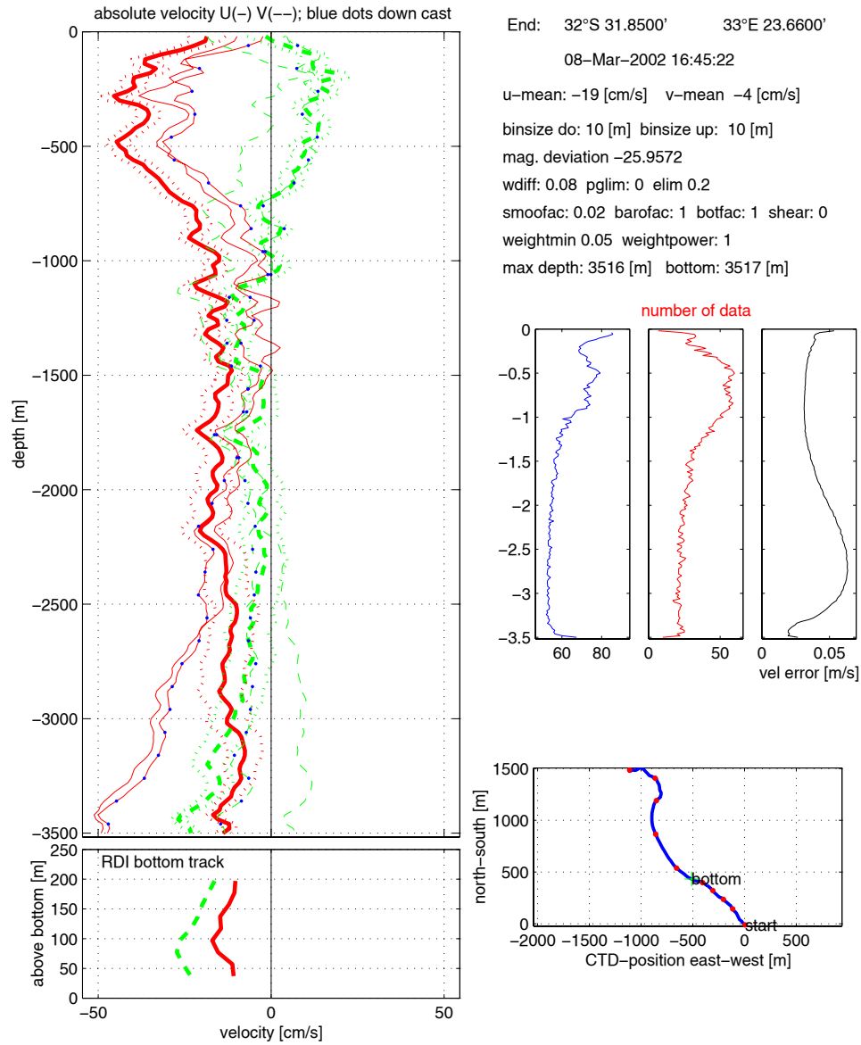
Figure L13: DWH velocity, data quality and ship drift processed using Visbeck method WITH bottom tracked velocity constraint
