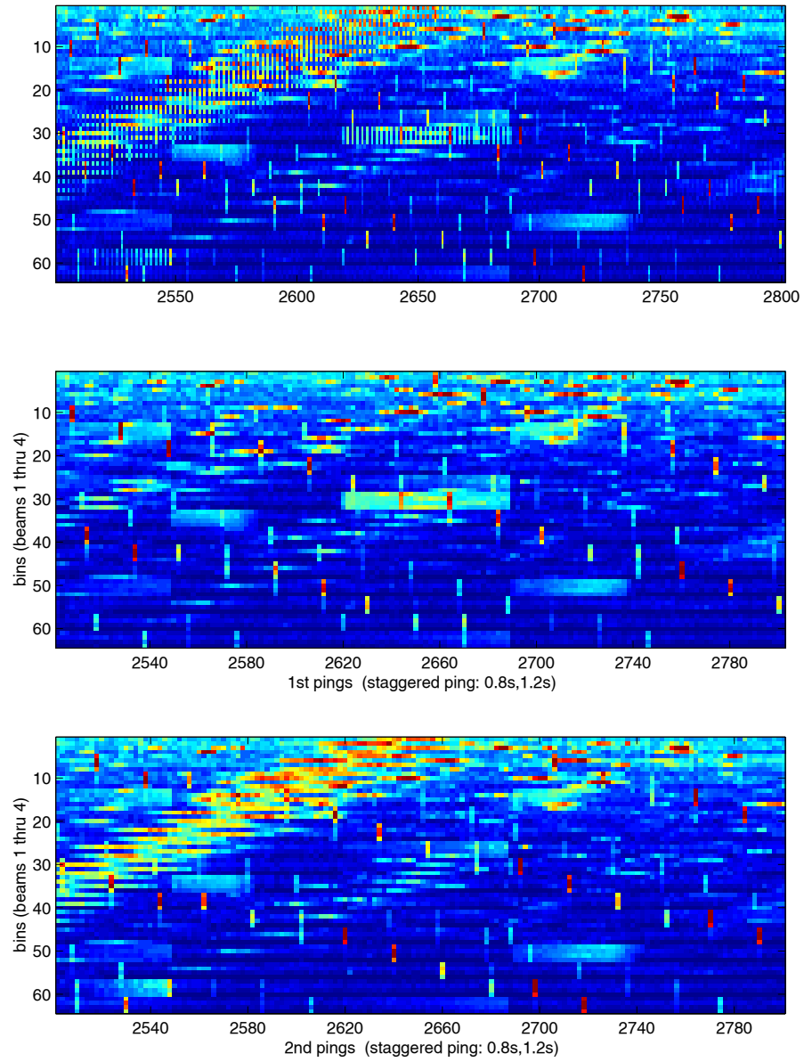
Figure L4: Combined BB and DWH deployment: Detail of Beam Amplitudes
