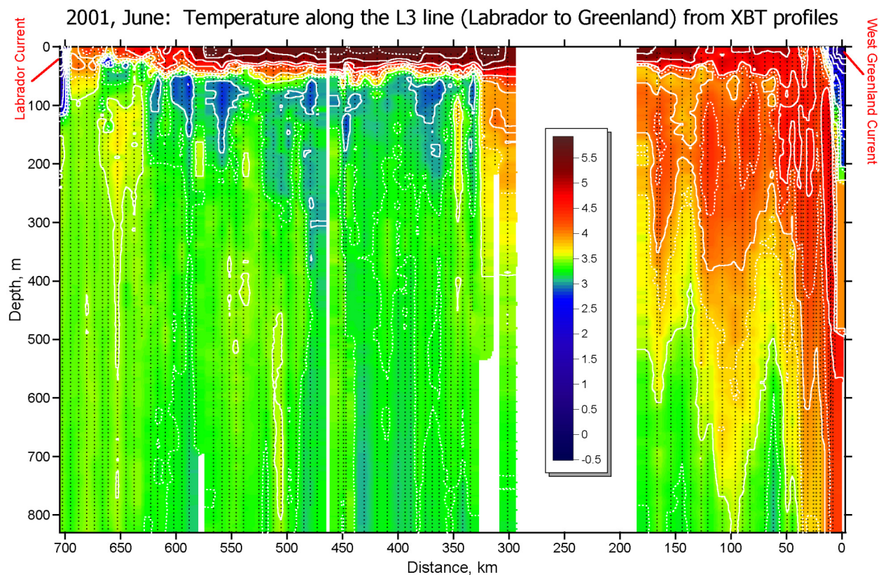
Figure 3. Section plot of preliminary XBT data along AR07W.
