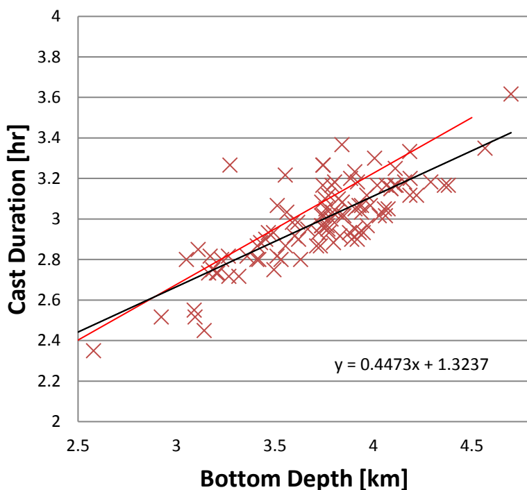
Figure 3. The length of time the CTD was on in the water plotted against the depth of the station for all casts on leg 1. The red x's and the black trend line and its equation reflect the actual times. The red line is the relationship expected at the outset of the project.
