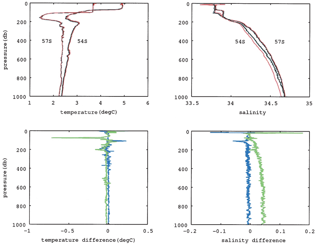
Fig. 5. Comparison between CTD and XCTD at 54 and 57°S. Left panels are for temperature and right for salinity. Red lines in the upper panels are CTD reference values, and black lines denote XCTD measurements. The lines in the lower panels show residuals (blue for 57°S and green for 54°S).
