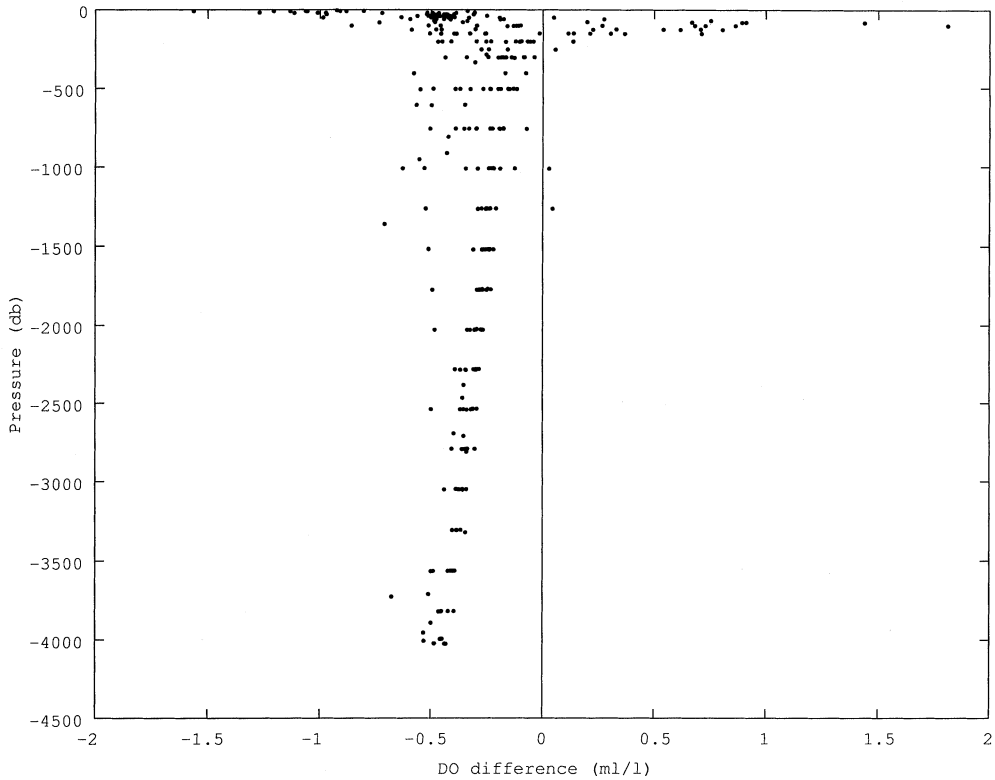
Fig. 4. Dissolved Oxygen residual ( DO (bottle)— DO (CTD))
