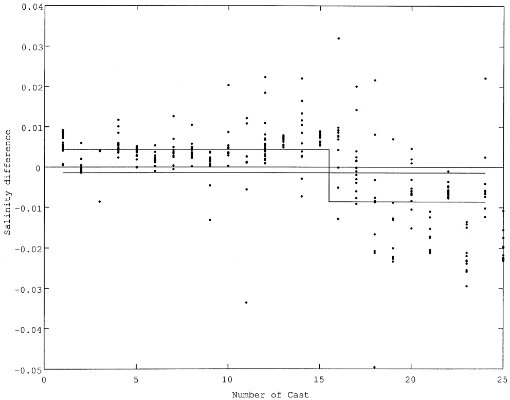
Fig. 3. Salinity residual (salinity (bottle)–salinity (CTD)). The straight solid line denotes the averaged difference for all samples, and the kinked line denotes the averaged level for casts 1 to 15 and for casts 16 to 25.
