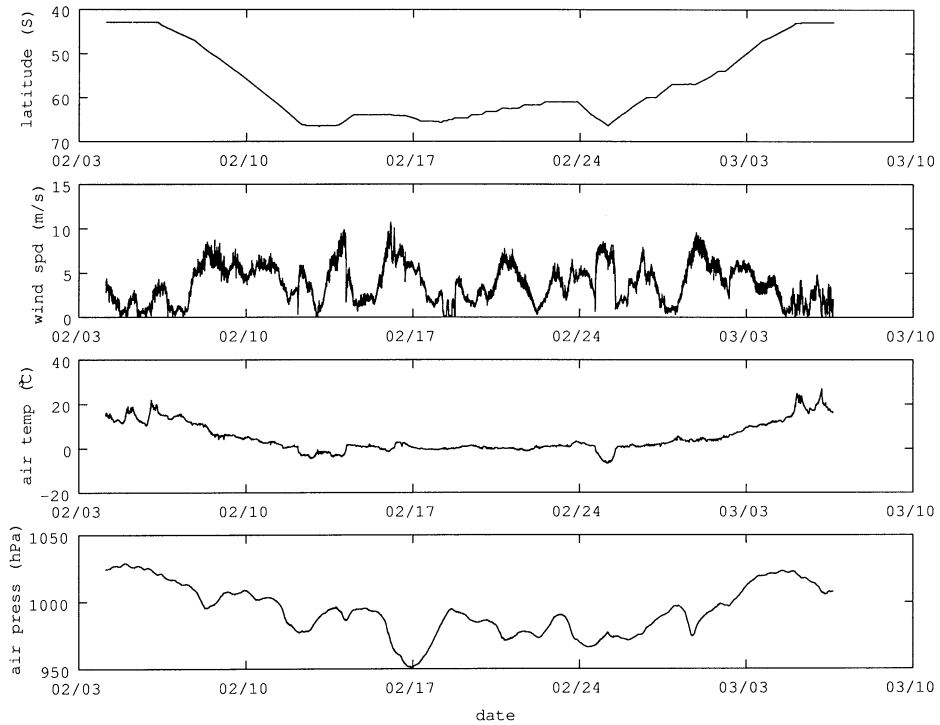
Fig. 2. Weather condition and meridional position during the cruise. a) latitude, b) wind speed (m/s), c) air temperature ( ^{\circ} C), and d) air pressure (hPa).
