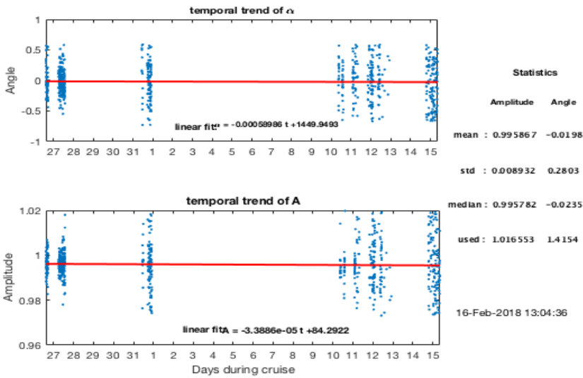
Figure 7: Misalignment angle and amplitude distributions after running the script with an initial misalignment angle of 1.4154° and an amplitude of 1.01655.
