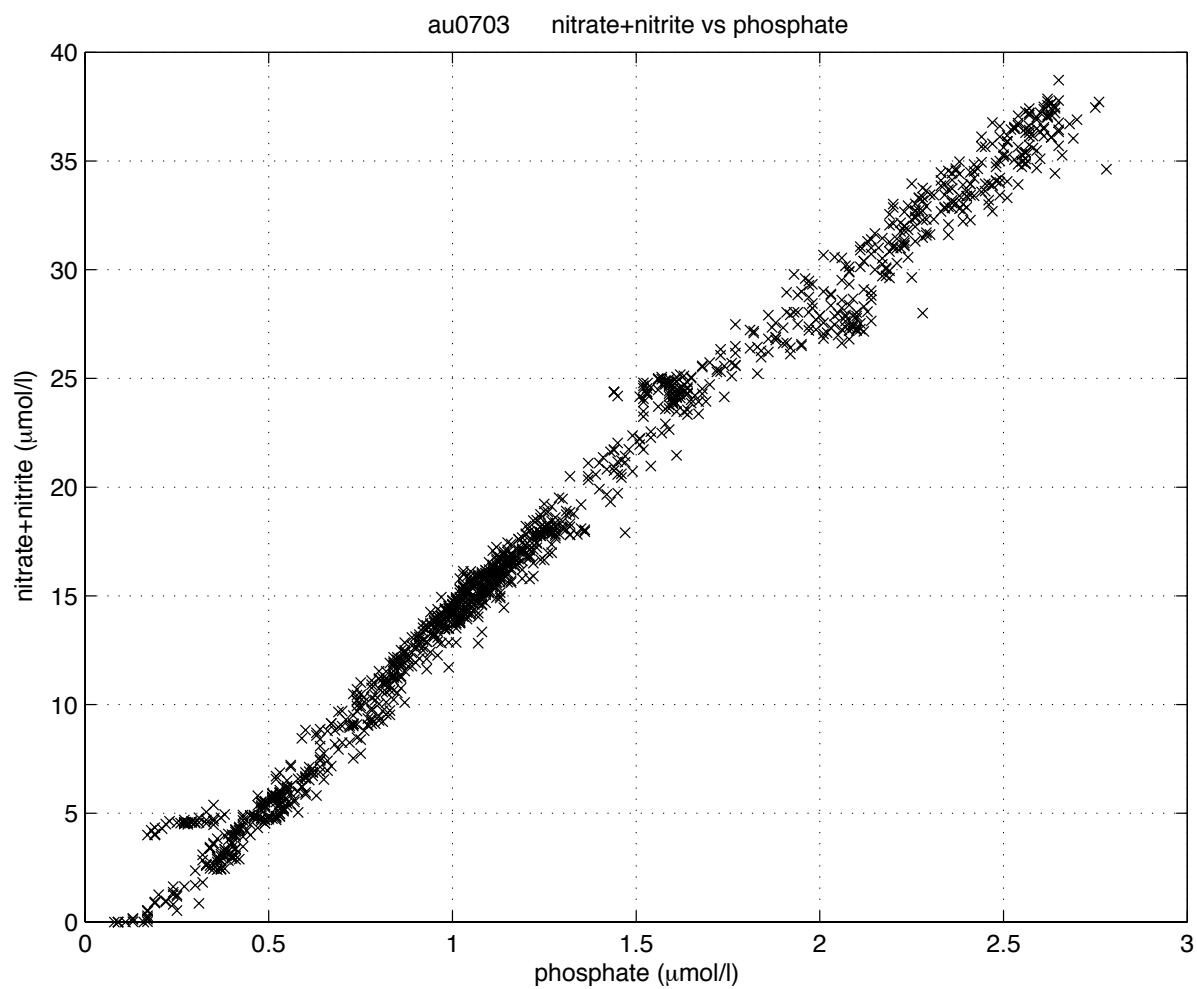
Figure 7: Nitrate+nitrite versus phosphate data for cruise au0703.
