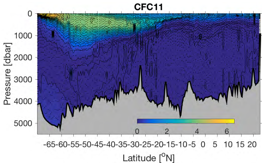
Figure 7d. The meridional – depth distribution of dissolved CFC-11 (pmol kg -1 ) along the 2016/17 P18 line in the South Pacific Ocean.
