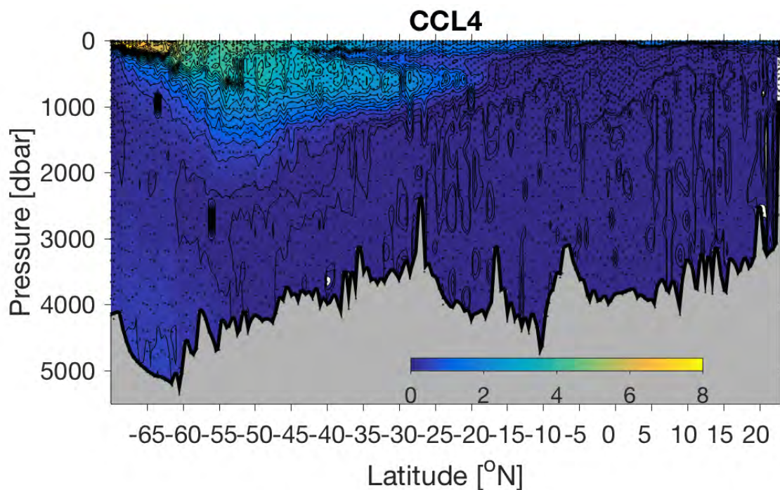
Figure 7e. The meridional – depth distribution of dissolved CCL 4 (pmol kg -1 ) along the 2016/17 P18 line in the South Pacific Ocean.
