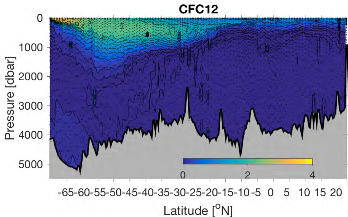
Figure 7c. The meridional – depth distribution of dissolved CFC-12 (pmol kg -1 ) along the 2016/17 P18 line in the South Pacific Ocean.
