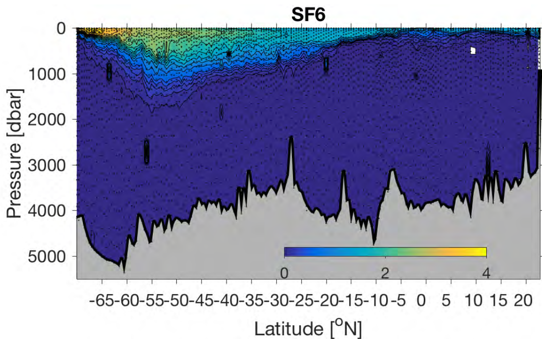
Figure 7f. The meridional – depth distribution of dissolved sulfur hexafluoride (fmol kg -1 ) along the 2016/17 P18 line in the South Pacific Ocean.
