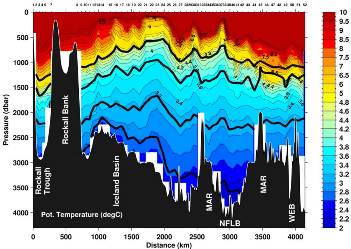
Figure 4.1: Potential Temperature (°C) as recorded during CTD casts. The displayed section follows the cruise track. Noted abbreviations are: MAR – Mid-Atlantic Ridge, NFLB – Newfoundland Basin, WEB – West European Basin. Solid black lines indicate the isopycnals \sigma_{\theta} = [27.68, 27.74, 27.80, 27.88] \text{ kg/m}^3 .
