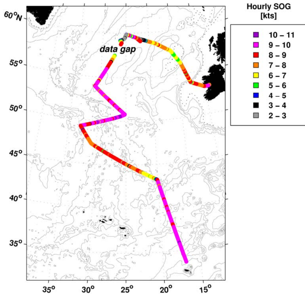
Figure 2.1: Speed over ground [knots] during R/V Pelagia cruise 64PE278. Available data were averaged to hourly values. Values below 2 knots have been omitted to exclude station work. Bathymetric contours are shown every 1000m with stippled lines indicating the 500m-isobath.
